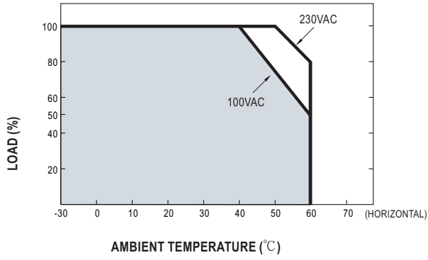
■ Derating Curve
